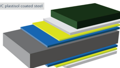
Plastisol top coat (200µm) Paint primer Pre treatment Zinc Steel
